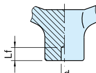
SH-C (下穴)
