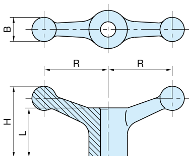
SH-R (精度穴)
