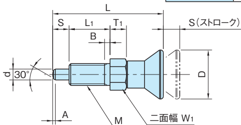
NDXNE NDXNE-SUS NDXNE-A-SUS
