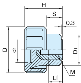
FTK FTK-SUS (メネジ)
