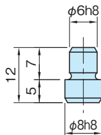
APS100-PIN
