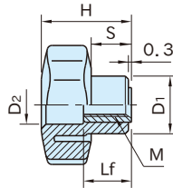
STK-NT (Tapped Through)
