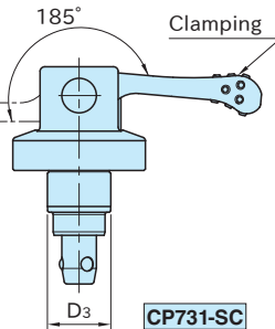
CP731-SC (Straight)
