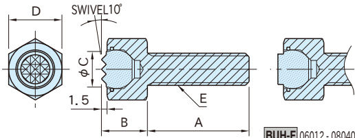
BUH-S 06012-08040 (Serrated, Steel Ball)
