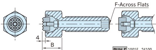
BUH-S 10015-24100 (Serrated, Steel Tip)
