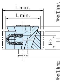
BK2-VT-F DK2-VT-F FK2-VT-F (Smooth Jaw)
