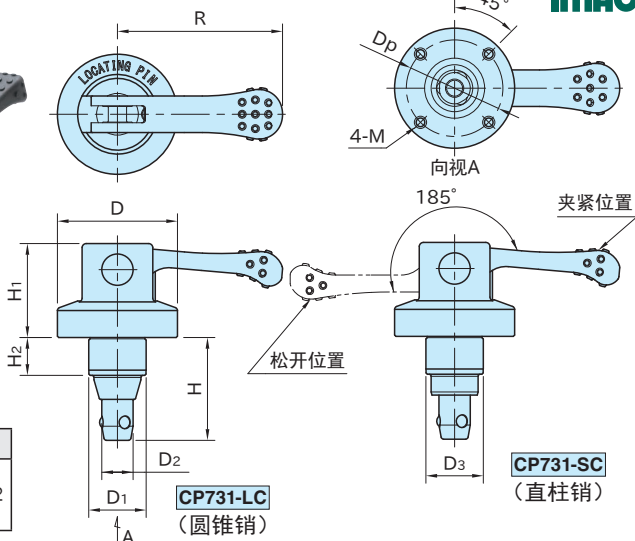
CP731-SC (直柱销)
