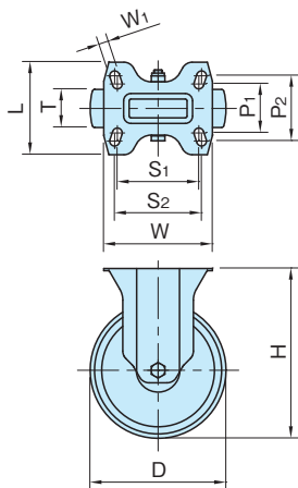
CAFF-PBL CAFF-PBL-SUS (固定)
