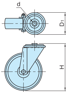
CAFF-FBL CAFF-FBL-SUS (旋回,通し穴)
